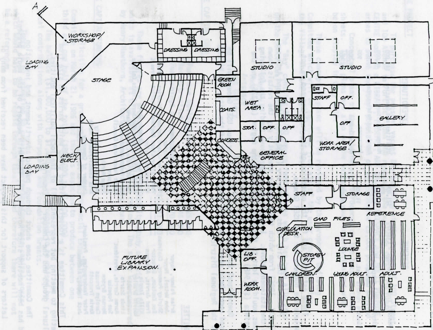
CONCEPT LOWER FLOOR PLAN
